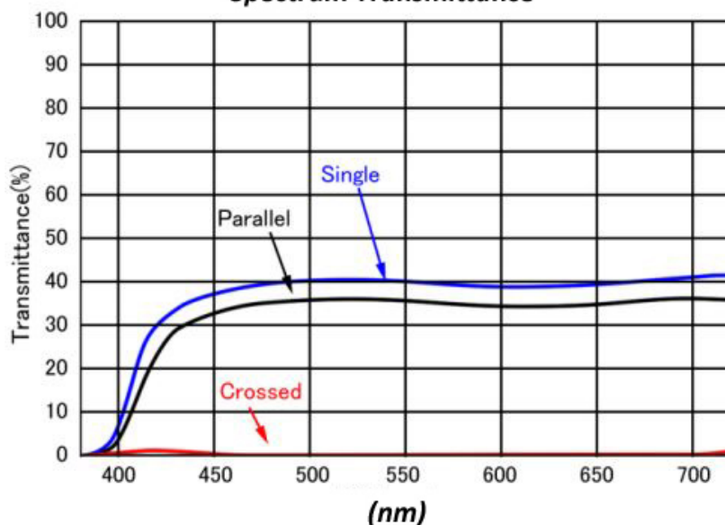
Spectrum Transmittance
