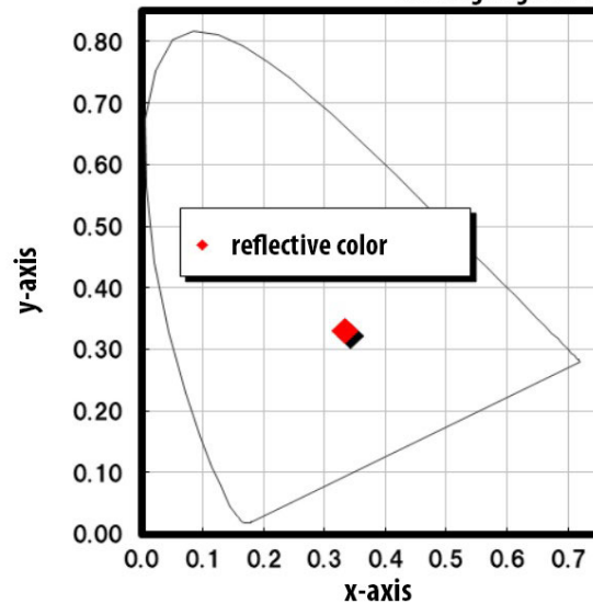
Color Characteristics : CIE1931 XYZ color system viewing angle 10 deg
