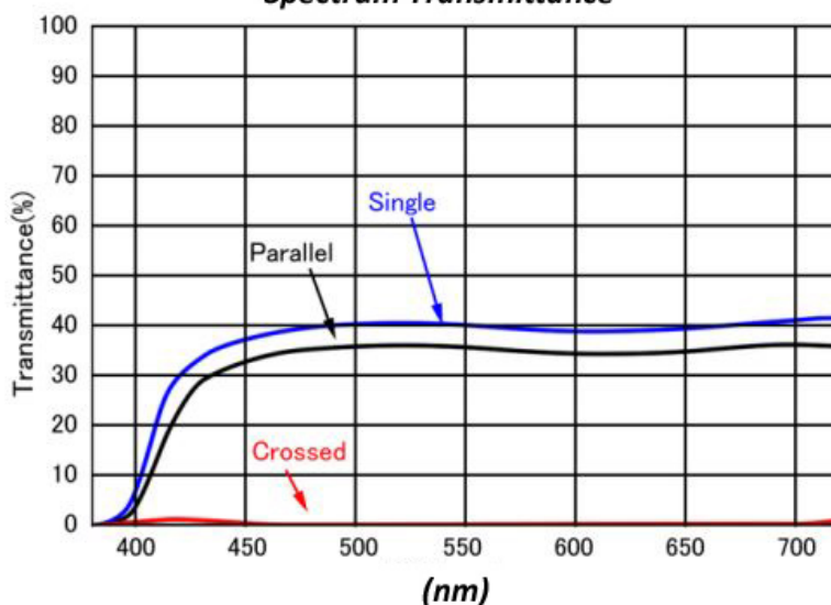
Spectrum Transmittance
